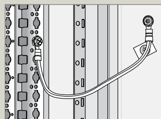
Internal earthing
