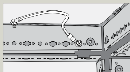
External earthing
