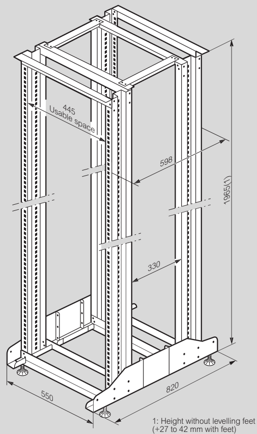
4-upright bati-rack Cat.No 0 463 96
