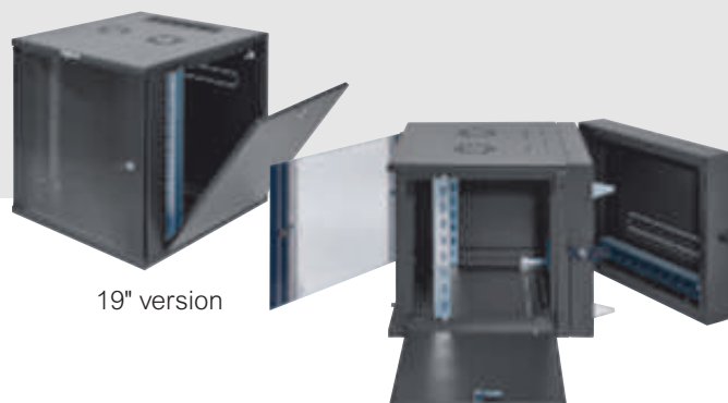
19" pivoting version
