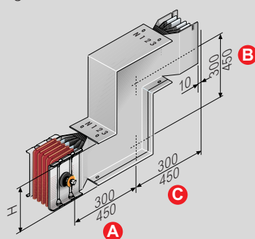
MIN AND MAX DIMENSIONS OF SINGLE AND DOUBLE BAR
