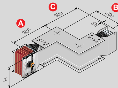
MIN AND MAX DIMENSIONS OF SINGLE AND DOUBLE BAR
