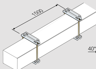
Flat installation
