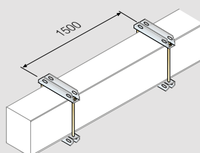
Edgewise installation
