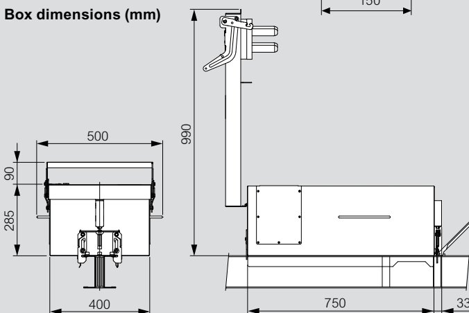
Box dimensions (mm)
