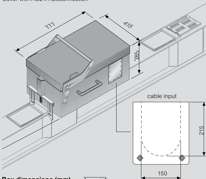
Box dimensions (mm)
