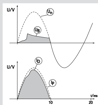
Zero point extinguishing MCB
