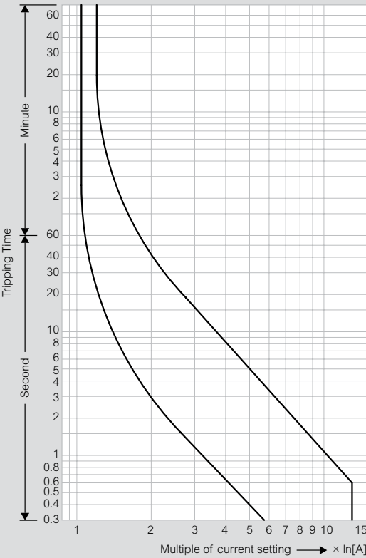
Hot starting
