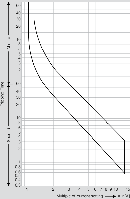
Cold starting
