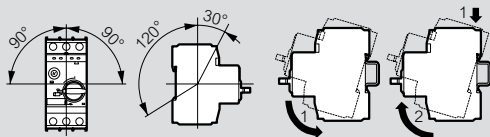
Operating positions
