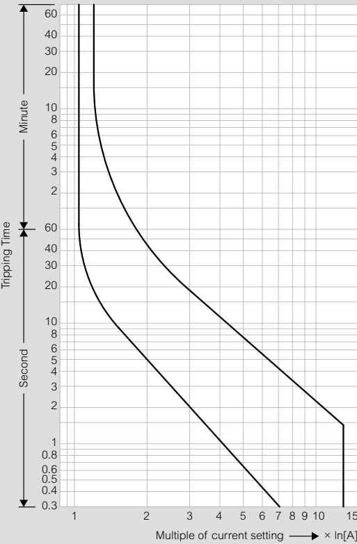
Hot starting
