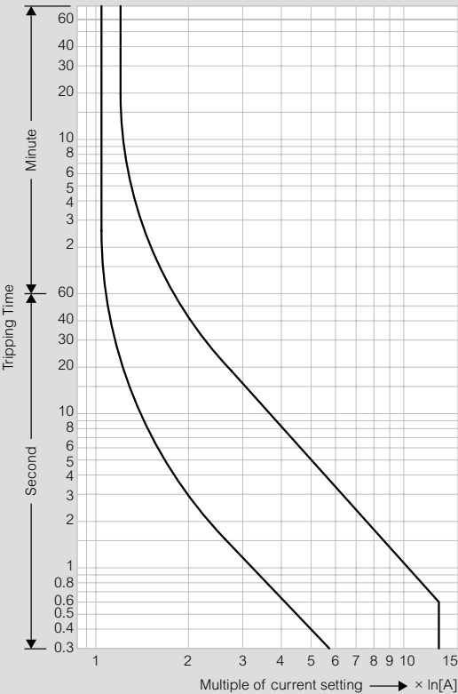
Hot starting
