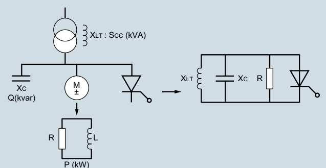
Schematic diagram
