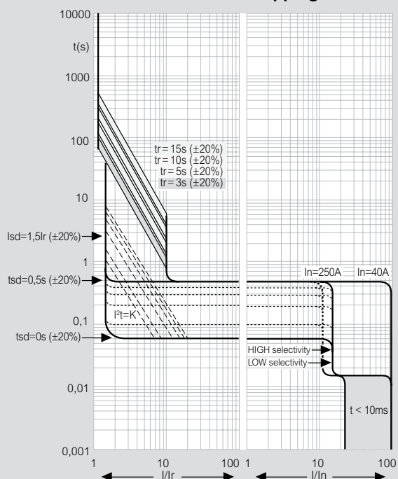
DPX 3 250 electronic release Tripping curves
