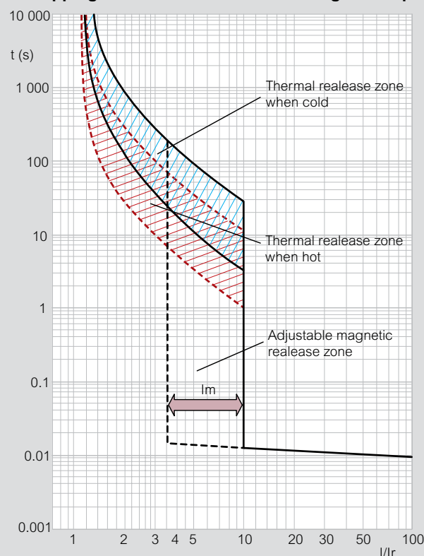
■ Tripping curve for a DPX 3 thermal-magnetic trip
